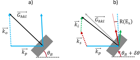
FIG. 1. Schematic illustration of pump-crystal interaction in the case of a) Bragg diffraction and b) parametric down-conversion, around the crystal reciprocal lattice vector with Miller Indices [hkl] . In the latter case, signal and idler photons are produced, with wavevectors \vec{k}_s and \vec{k}_i . The dotted lines indicate the vector calculations. Figure is adapted from [12].
