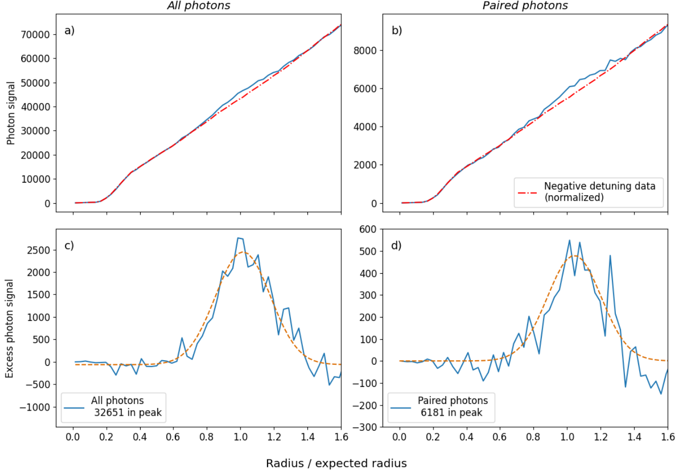
FIG. 5. Signal histograms as a function of normalized radius ( r/r_{exp} ), across the energy range 3.9 – 5.9 keV. The upper figures show the signal for all photons, in a), and paired photons, in b), with the background (negatively detuned) signal normalized to each. The lower figures show the difference between the signal and background in the respective upper figures. The Gaussian peak is fitted to the excess signal from down-converted pairs as a guide to the eye.
