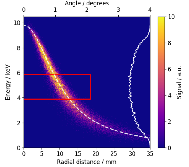
FIG. 2. Simulated down-conversion data, assuming an energy spread of \Delta E/E = 1 \times 10^{-4} . The red outline shows the coverage analyzed in this experiment, and the dashed white line shows the expected radial distance for each energy, r_{exp} , defined in Equation 4. The solid white line shows the total signal at each photon energy, demonstrating the higher probability of down conversion near to an even energy split.
