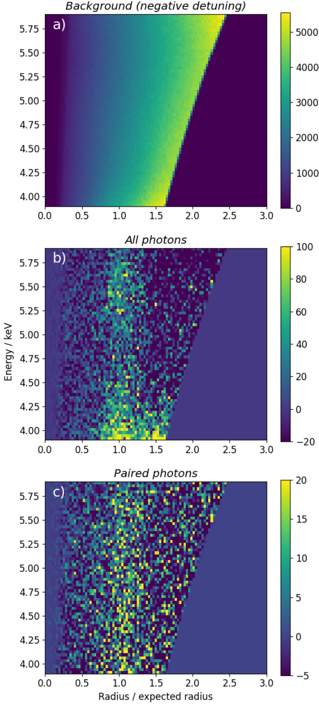
FIG. 4. Observed signal as a function of photon energy vs. distance from detector center, relative to the expected distance for that energy. a) Shows the background signal, with the crystal detuned to negative angles, such that down-conversion is not possible. The lower two images show the excess signal over that background with positive detuning ( \delta\theta = 12 mdeg) before, b), and after, c), photon pair-finding. In both, the peak at r/r_{exp} = 1 corresponds to down-converted photons. The color bar represents photons per bin - note the difference for each figure.
