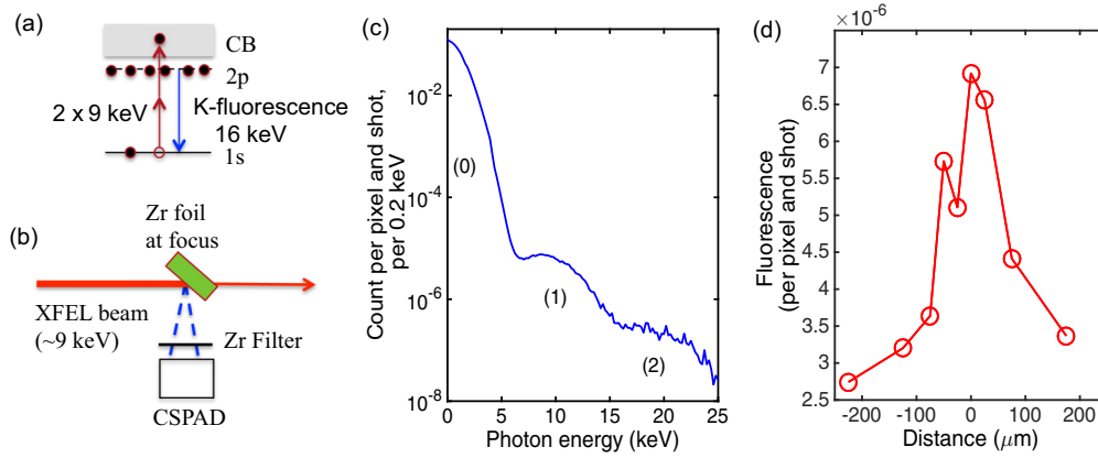
FIG. 1. (a) Schematic for nonsequential two-photon K -shell absorption in metallic Zr. When the incident photon energy exceeds half the single-photon K -absorption threshold ( \sim 18 keV), a 1s vacancy can be created through the simultaneous absorption of two (or more) photons. This vacancy is primarily filled by radiative decay from the 2p state in the form of K_{\alpha} fluorescence. (b) A powerful XFEL beam near 9 keV is focused to a submicron spot on a 25\text{-}\mu\text{m} thin Zr foil. The fluorescent signal is collected at 90^\circ in the polarization plane using a 140-K pixel single-photon-sensitive detector. A 50\text{-}\mu\text{m} Zr filter is inserted in front of the detector to reduce the background from scattered photons. (c) A representative detector histogram accumulated over 3000 shots, where peaks (0), (1), and (2) correspond to pixels registering zero photons, single photons near the fundamental ( \sim 9 keV), and single photons near the K -fluorescence peak ( \sim 16 keV), respectively, for an incident pulse energy of \sim 10 \mu\text{J} . The background from the pileup from two 9-keV photons in a single pixel has been suppressed as described in the text. (d) Dependence of peak (2) as the sample is scanned through the focal plane.
